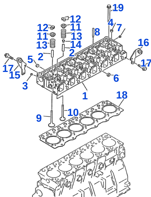
Fig. 101 CYLINDER HEAD
