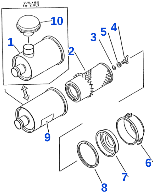
Fig. 131 AIR CLEANER
