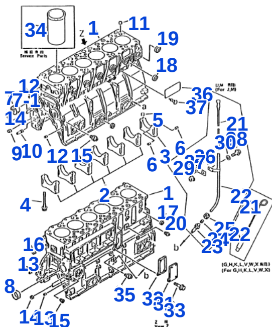
Fig. 202 CYLINDER BLOCK (G,H,I,J,K,L,M,V,W,X)
