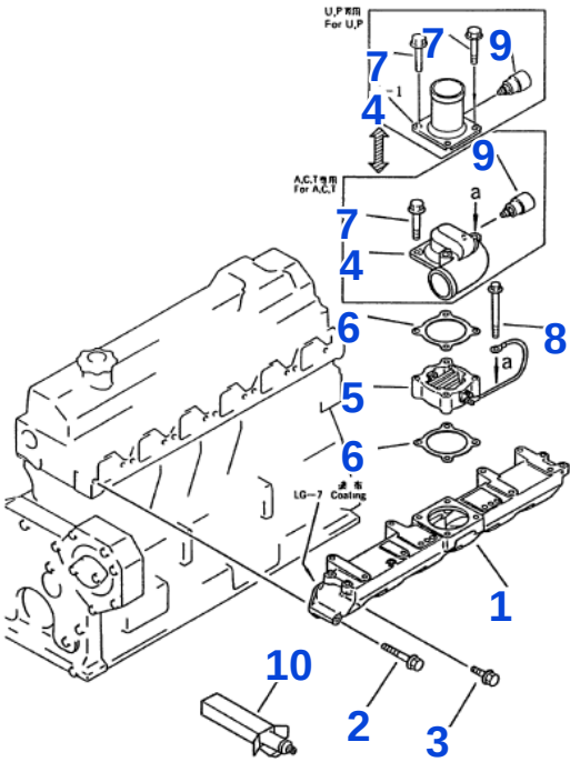
Fig. 111 AIR INTAKE MANIFOLD AND CONNECTION (A,C,T,U,P)
