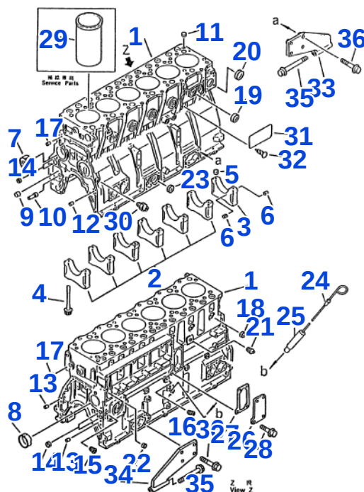
Fig. 201 CYLINDER BLOCK (A,C)
