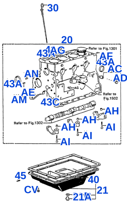
FIG.1105 CYLINDER BLOCK
