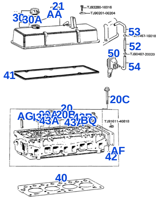
FIG.1104 CYLINDER HEAD & VENTILATION HOSE
