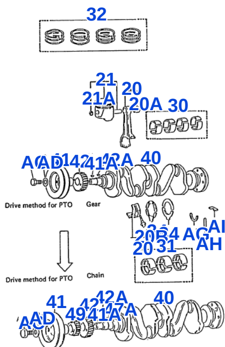
FIG.1301 CRANKSHAFT & PISTON
