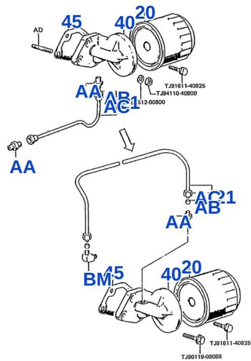
FIG.1502 OIL FILTER
