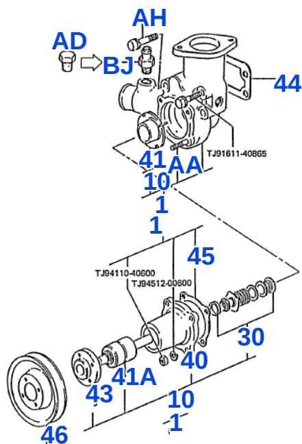
FIG.1601 WATER PUMP
