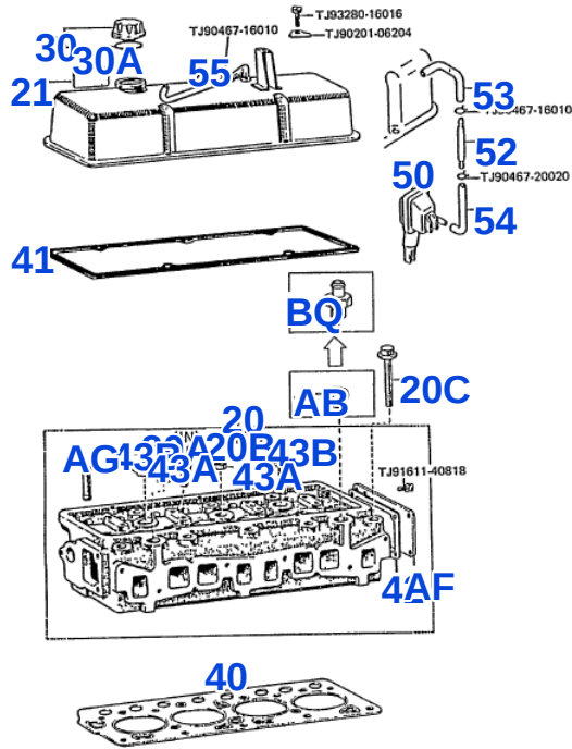
FIG.1104 CYLINDER HEAD & VENTILATION HOSE
