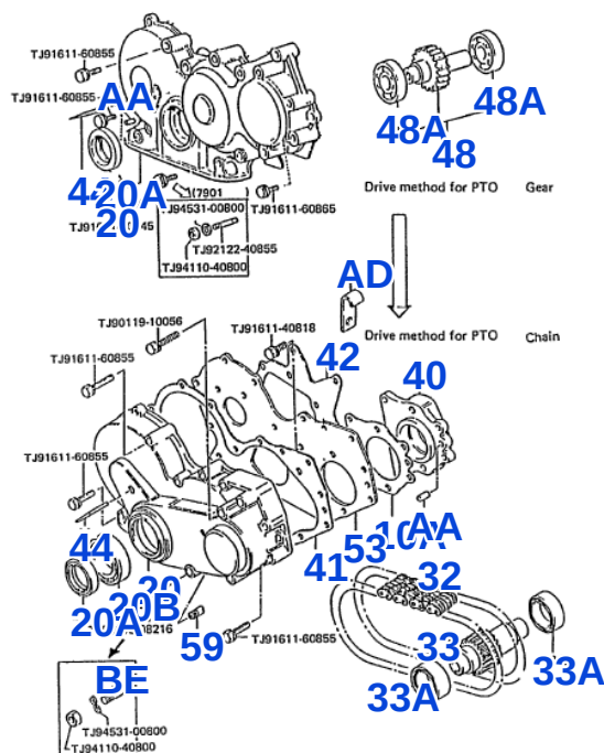
FIG.1106 TIMING GEAR COVER & END PLATE
