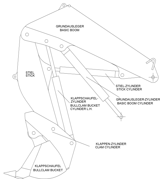
Klappschaufel-Einrichtung (KSE) Bullclam Bucket Equipment (BBE)
