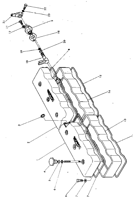
Fig. 102 CYLINDER HEAD COVER
