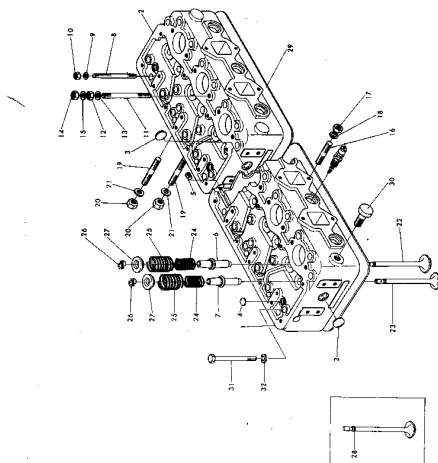
Fig.101 CYLINDER HEAD
