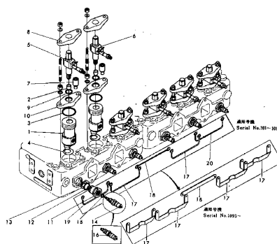
Fig. 103 PRECOMBUSTION CHAMBER
