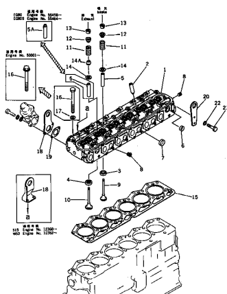
FIG. 101 CYLINDER HEAD
