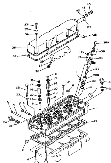
FIG. 101 CYLINDER HEAD
