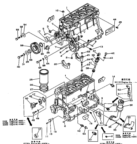
FIG. 202 CYLINDER BLOCK
