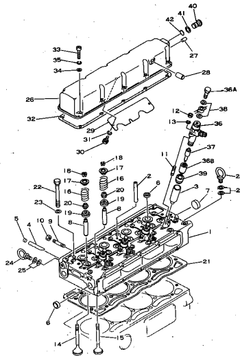
FIG. 101 CYLINDER HEAD
