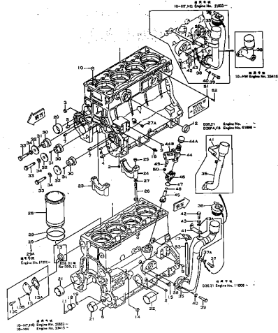
FIG. 201 CYLINDER BLOCK
