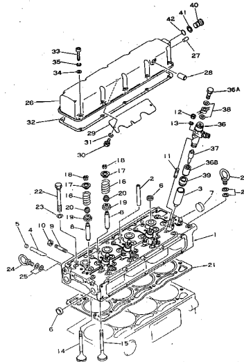
FIG. 101 CYLINDER HEAD
