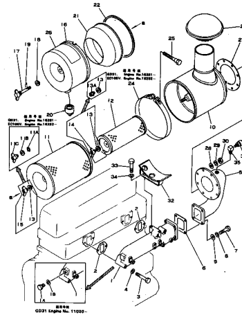
FIG. 111 AIR INTAKE MANIFOLD AND AIR CLEANER
