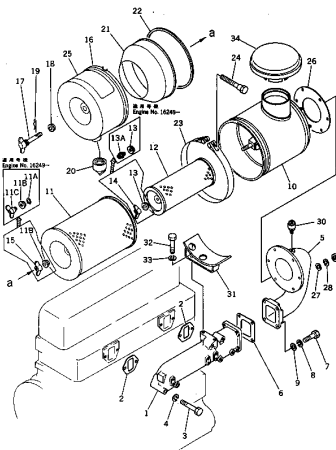
FIG. 113 AIR INTAKE MANIFOLD AND AIR CLEANER
