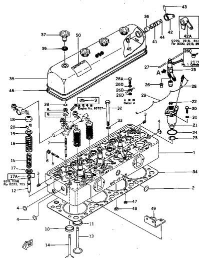
FIG. 1101 CYLINDER HEAD, COVER AND PRECOMBUSTION CHAMBER
