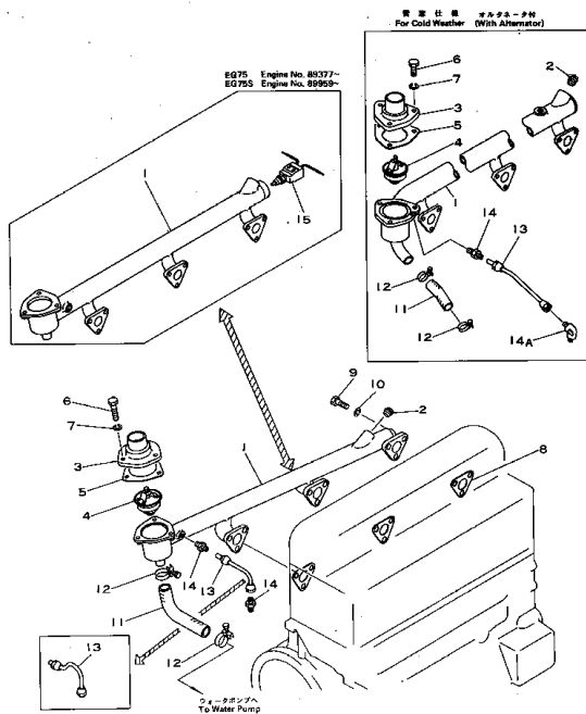
FIG. 1131 WATER MANIFOLD AND THERMOSTAT
