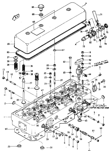
Fig. 101 CYLINDER HEAD, PRECOMBUSTION CHAMBER AND COMPRESSION RELEASE (1/2) (Engine No. 1301~30254)
