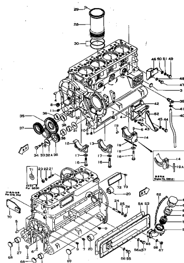
FIG. 1201 CYLINDER BLOCK
