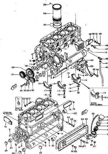
FIG. 1201 CYLINDER BLOCK
