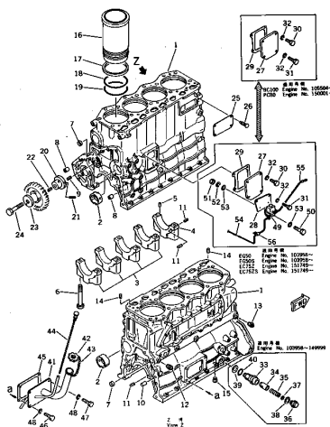
FIG. 2202 CYLINDER BLOCK
