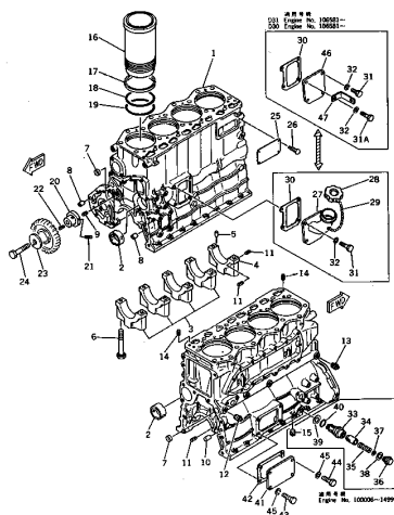
FIG. 2201 CYLINDER BLOCK
