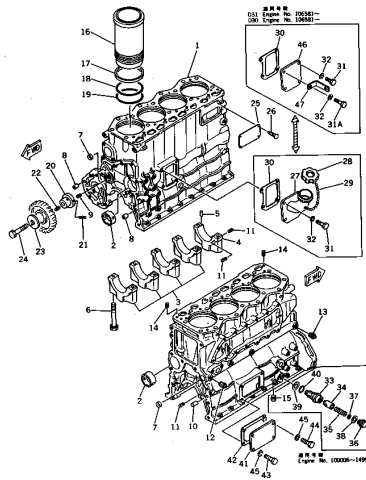
FIG. 2201 CYLINDER BLOCK
