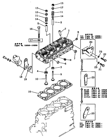
FIG. 2101 CYLINDER HEAD
