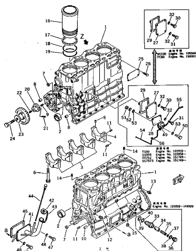
FIG. 2202 CYLINDER BLOCK
