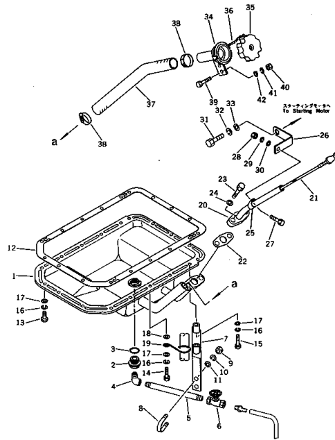
FIG. 217 OIL PAN (EC35ZS ENGINE NO. 11852- )
