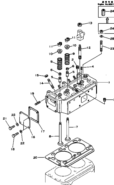
Fig. 101 CYLINDER HEAD
