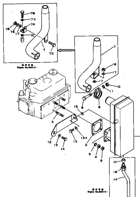
Fig. 121 EXHAUST MANIFOLD AND SILENCER
