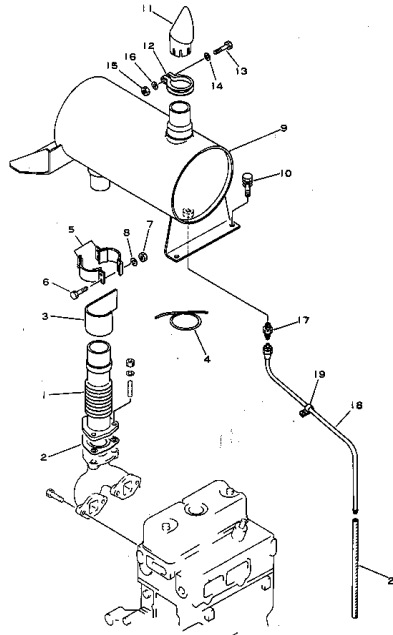
FIG. 1187 MUFFLER (EC25ZS ENGINE NO. 23012 - )
