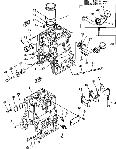
FIG. 1202 CYLINDER BLOCK
