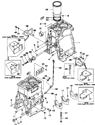
Fig. 201 CYLINDER BLOCK (D10 Engine No. 11225-~) (PC02 Engine No. 16531-~)
