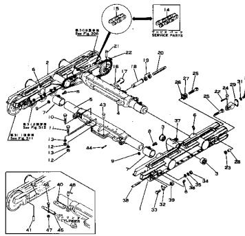
Fig.305 CRAWLER FRAME (25-BSC)
