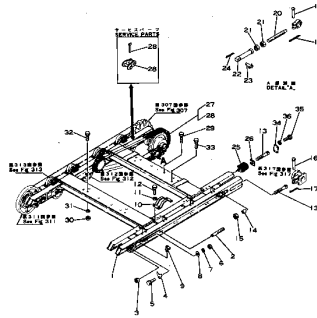
Fig. 304 CRAWLER FRAME (25-BHD)
