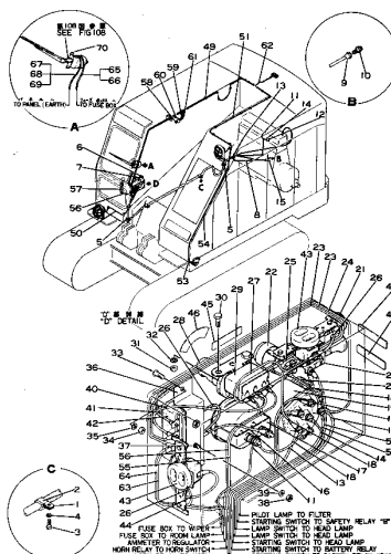
Fig. 105 ELECTRICAL SYSTEM (1/2)
