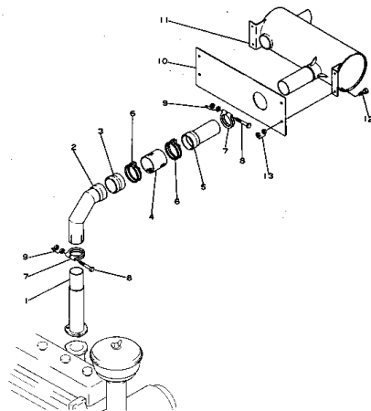
Fig.102A EXHAUST LINE (適用考慮) (Serial No.1094~ )
