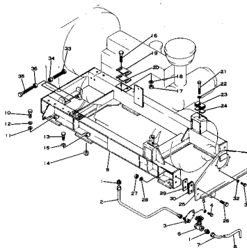
Fig.101A ENGINE ATTACHING PARTS (Serial No.1094~ )
