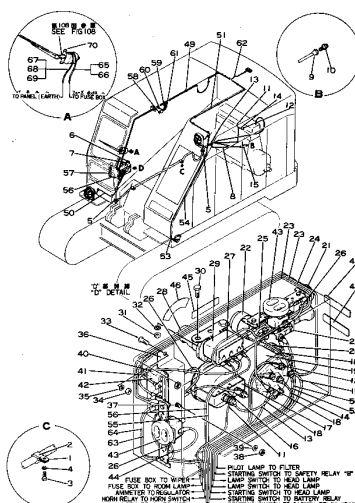
Fig. 105 ELECTRICAL SYSTEM (1/2)
