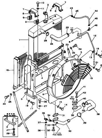
Fig. 1131 RADIATOR AND OIL COOLER
