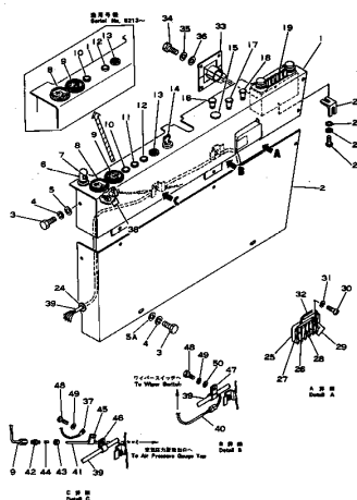
Fig. 1155 INSTRUMENT PANEL
