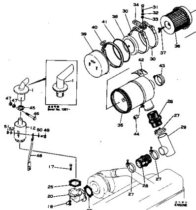
Fig. 102 AIR INTAKE AND EXHAUST LINE (Serial No. 1003-1286)
