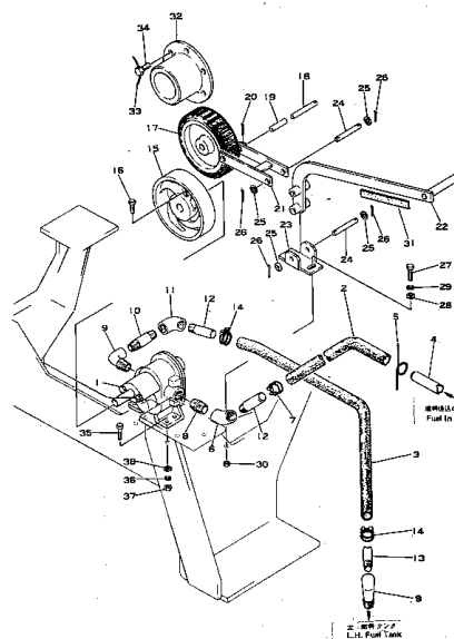
燃料給油装置 (適用機種) Fig. 105A FUEL FILLER SYSTEM (Serial No. 5001 ~)
