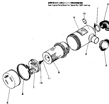
Fig. 102 AIR CLEANER (Serial No. 1001~5000)
