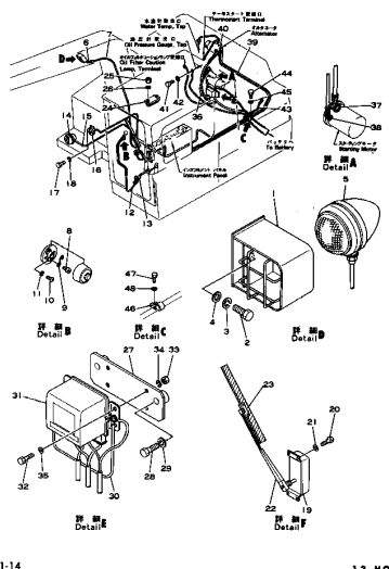
Fig. 106 LIGHTING SYSTEM
