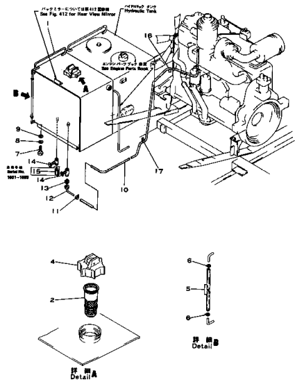
Fig. 104 FUEL TANK AND PIPING
