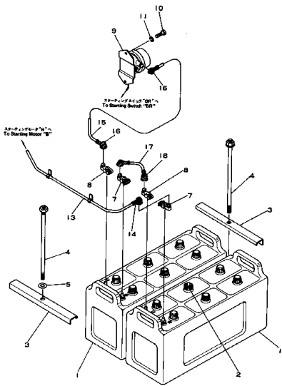
Fig. 105 BATTERY AND RELAY SWITCH
