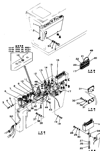
Fig. 1155 INSTRUMENT PANEL
