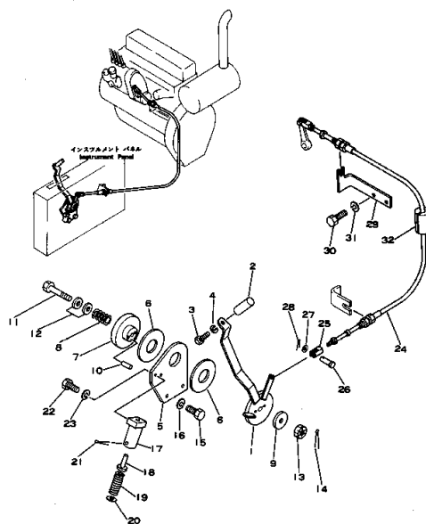
Fig. 1121A FUEL CONTROL LEVER AND LINKAGE 適用機種 (10-HT Serial No. 9501～) (10-HL Serial No. 6201～)
