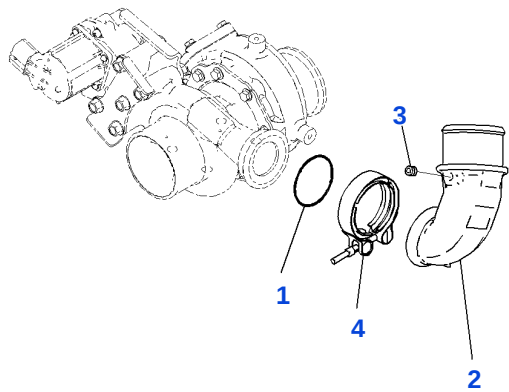
Variable Flow Turbocharger
