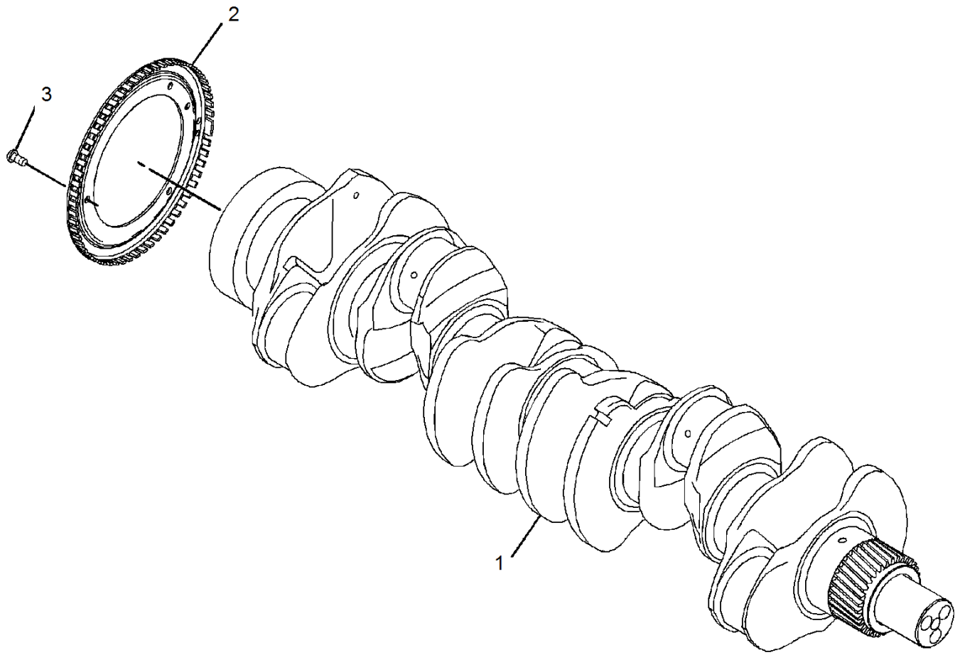
Drawing 1 of 1
