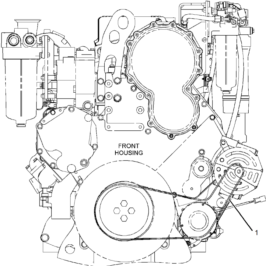
FRONT VIEW OF ENGINE
