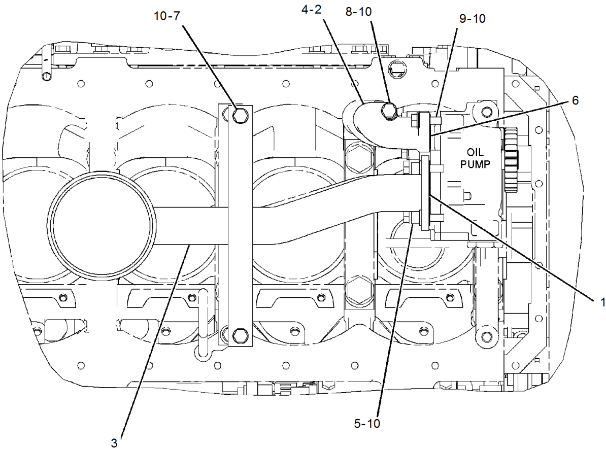
BOTTOM VIEW OF ENGINE
