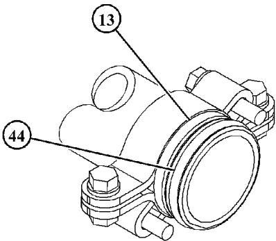
VIEW OF AREA L (PARTS REMOVED FOR CLARITY)
