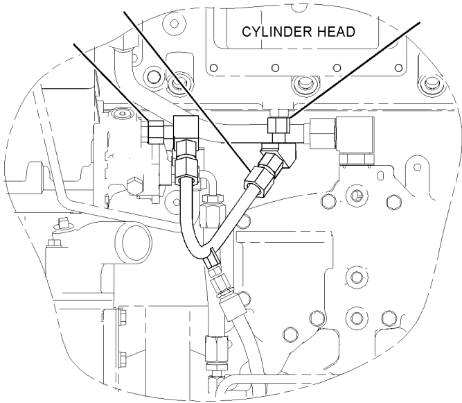
LEFT SIDE VIEW OF ENGINE
