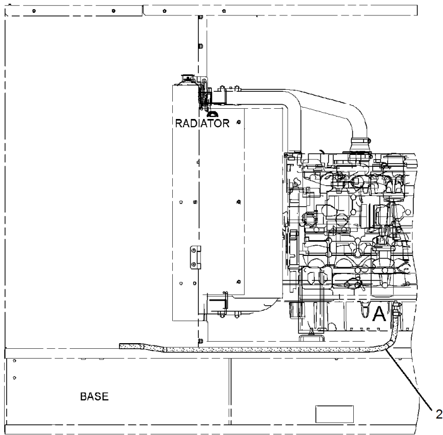
LEFT SIDE VIEW OF ENGINE
