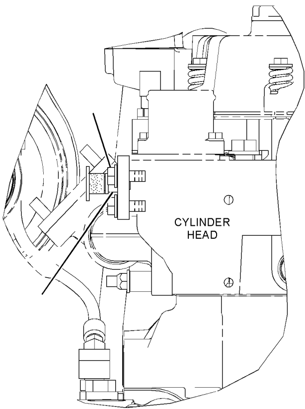
FRONT VIEW OF ENGINE
