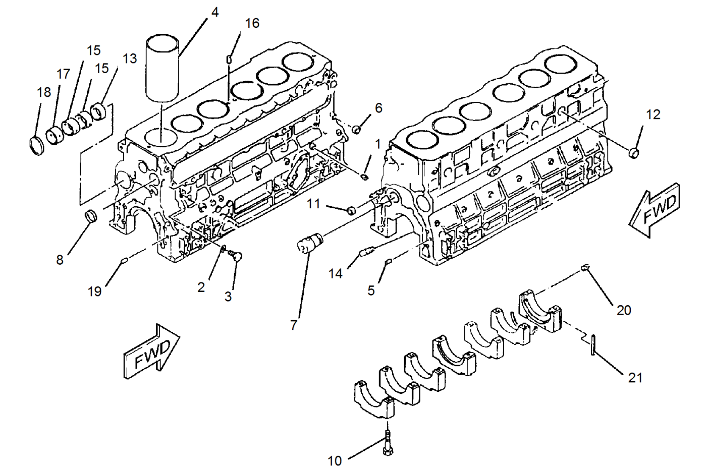
Drawing 1 of 1
