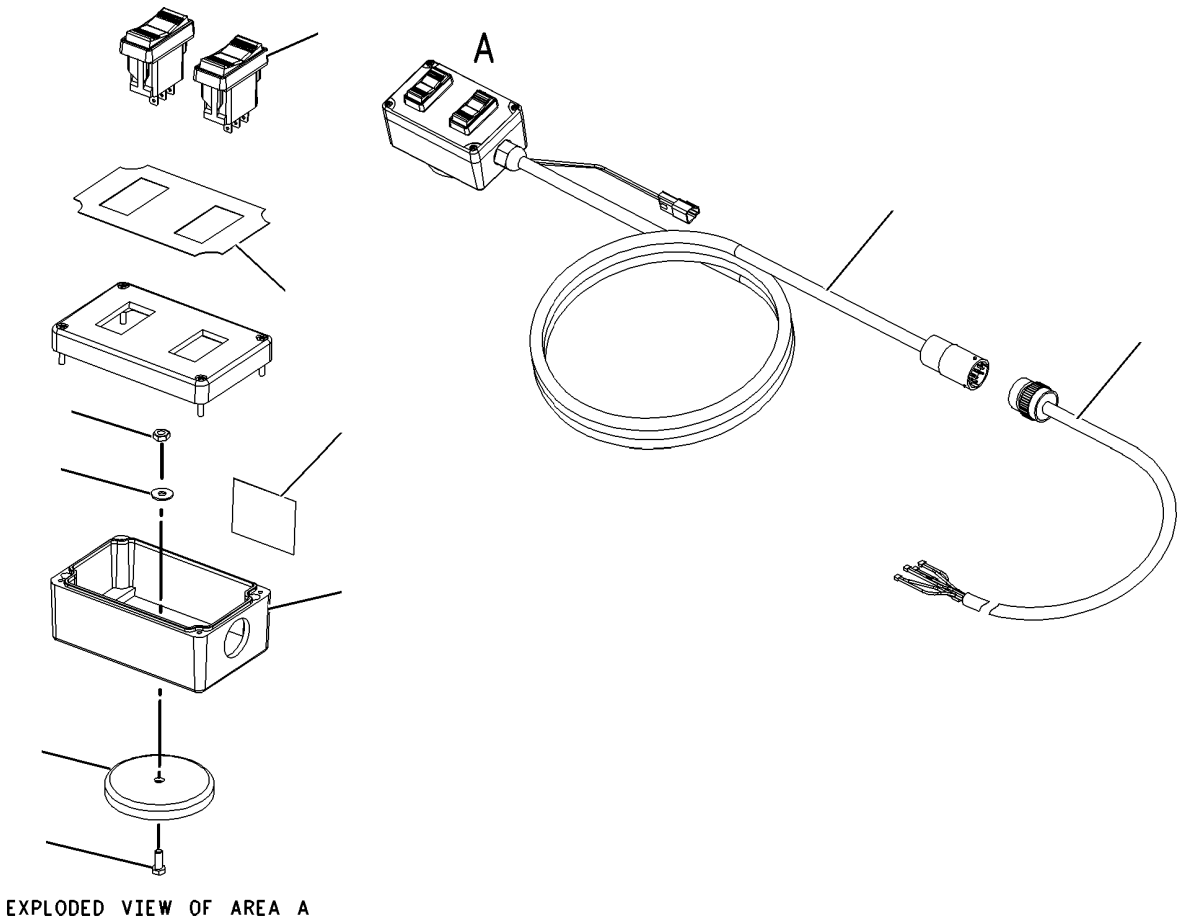
EXPLODED VIEW OF AREA A
