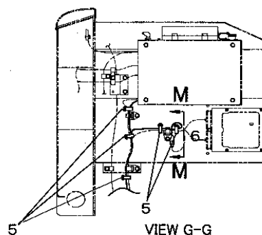
VIEW G-G
