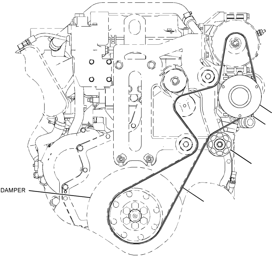
FRONT SIDE VIEW OF ENGINE
