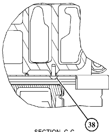
SECTION C-C
