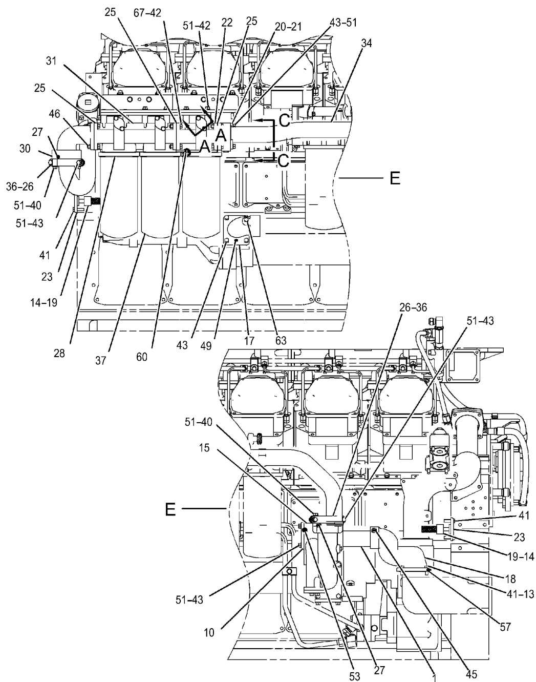
RIGHT SIDE VIEW OF ENGINE
