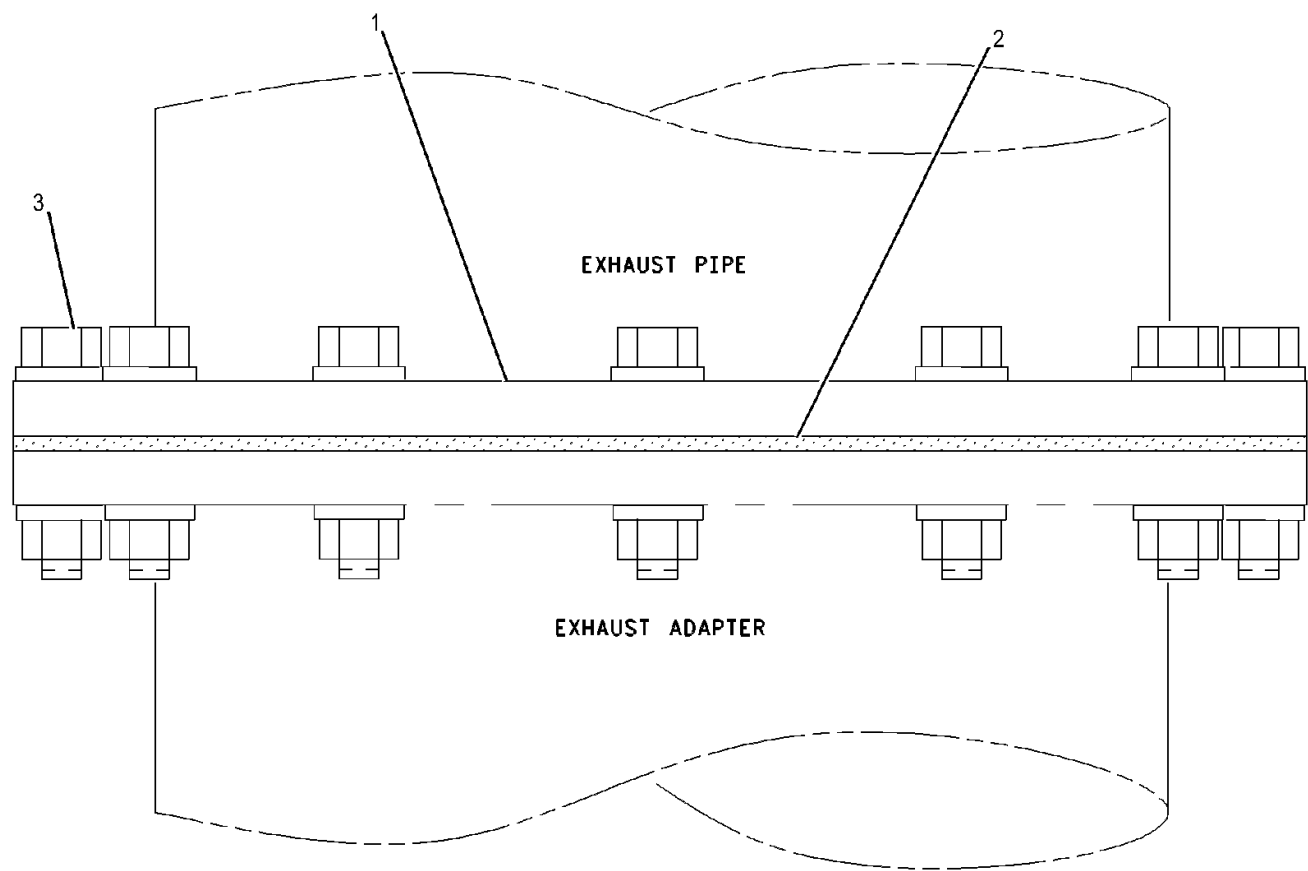
Drawing 1 of 1
