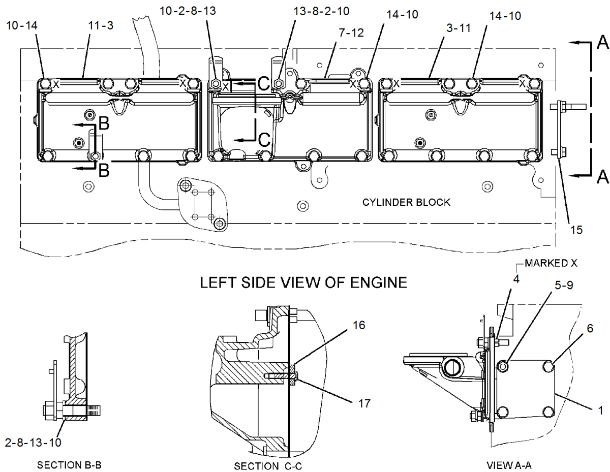
Drawing 1 of 1
